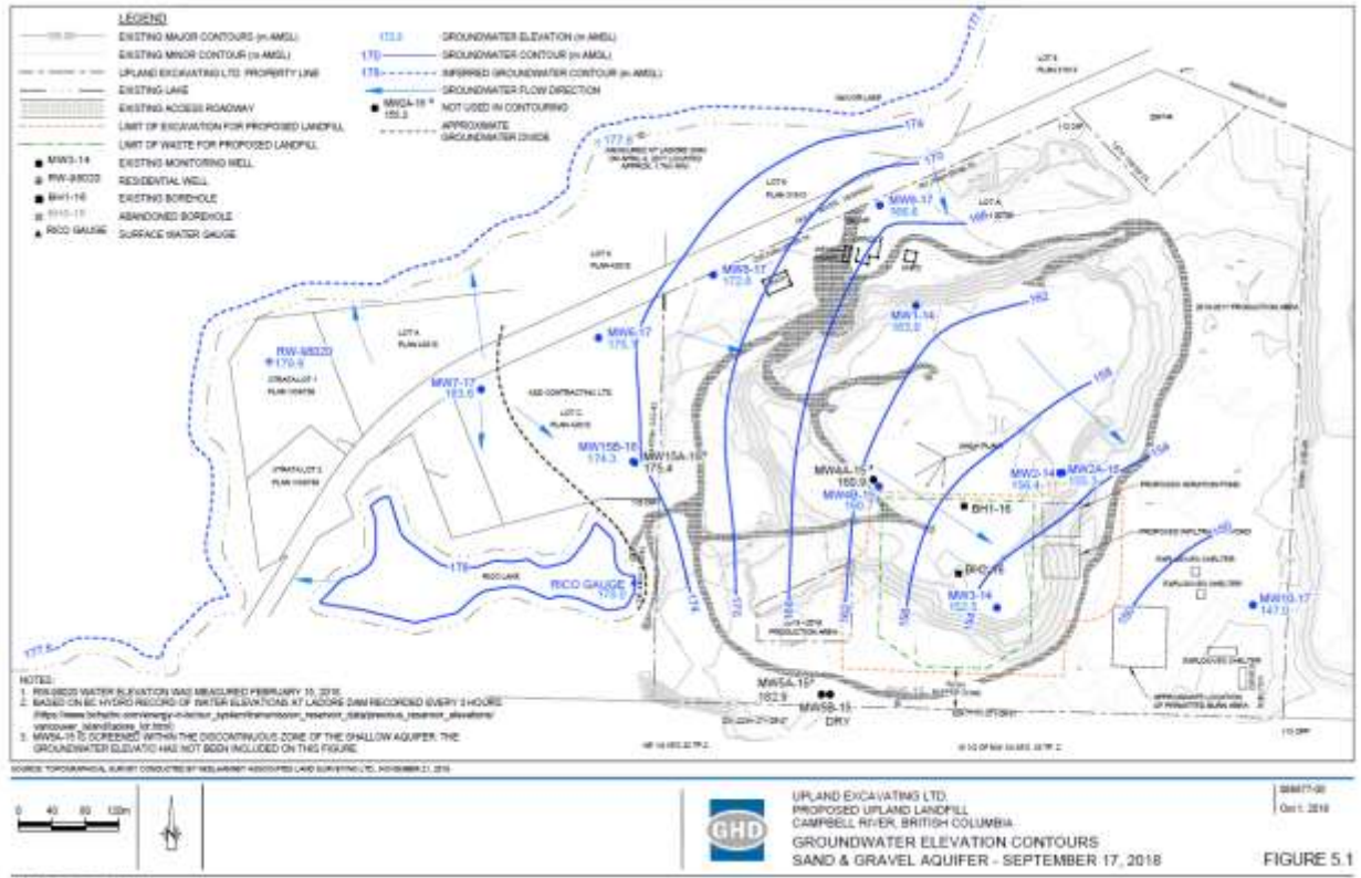
Figure 1. Water-level contours prepared by GHD, September 17, 2018 (from Figure 5.1, GD Response Letter Task 7).
