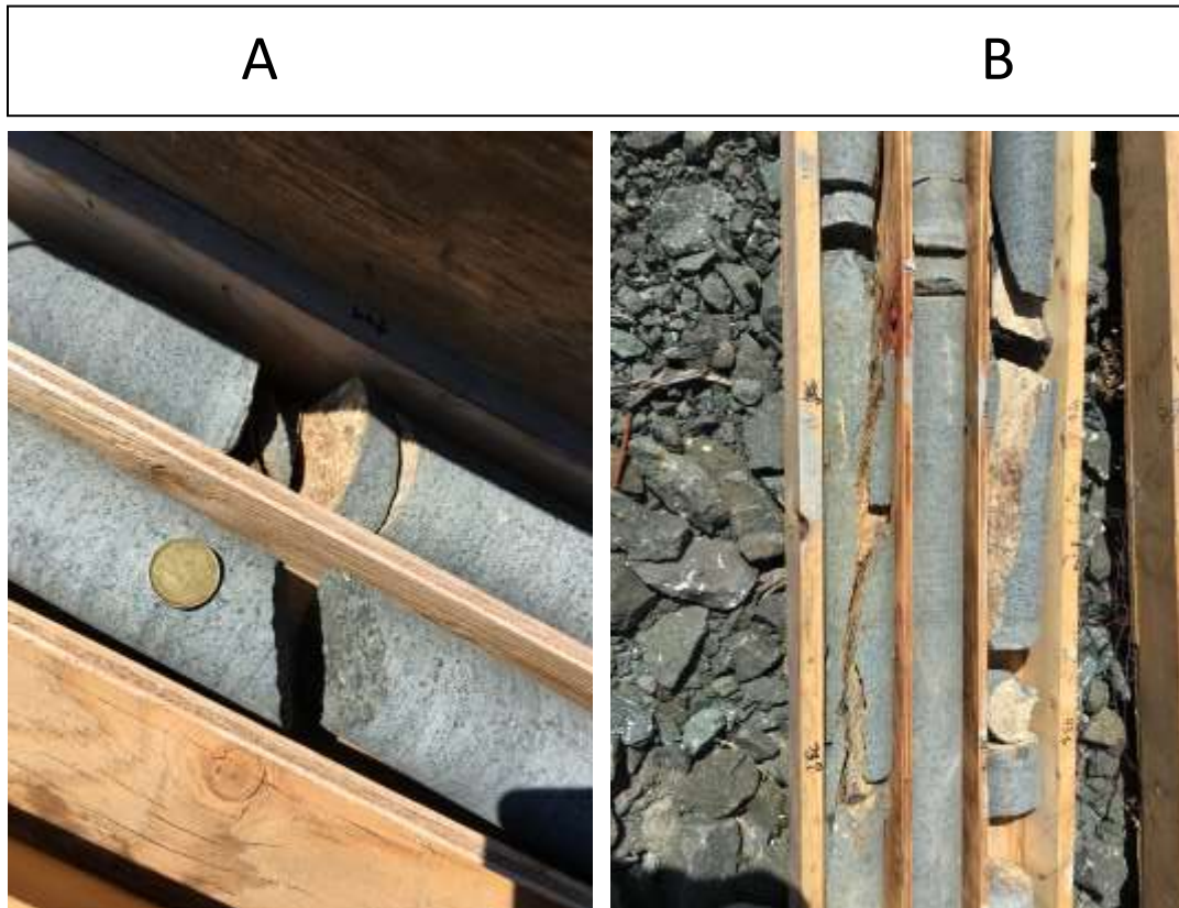
Figure 3. A) Rock core from MW15A-18 showing a weathered horizontal fracture (light brown weathered surface), and an unweathered fracture that probably resulted from coring. B) Weathered sub-vertical fractures in core from MW15A-18.
